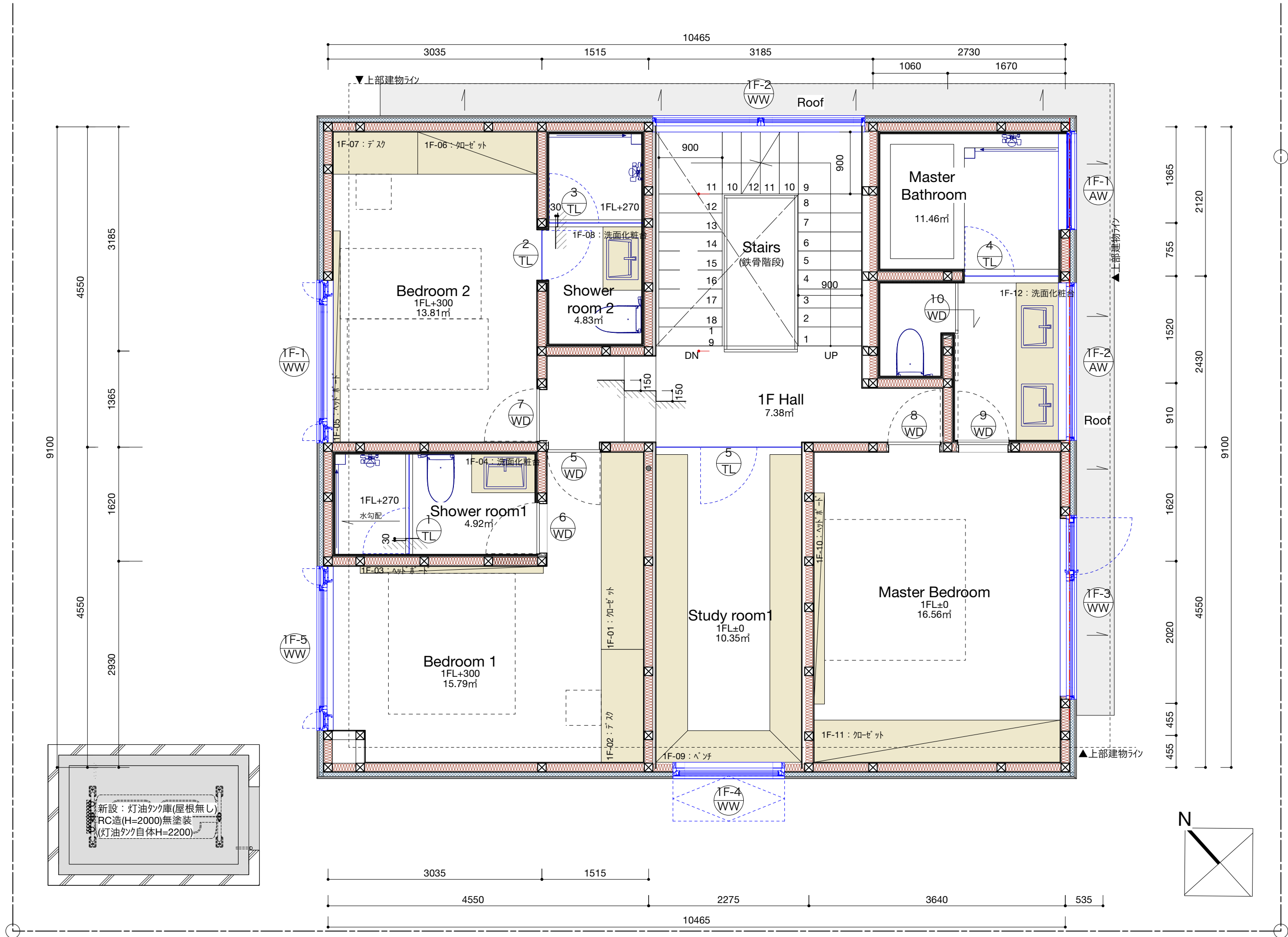
1F PLAN
